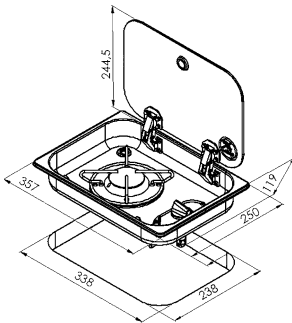
70568 1,80 kW 1 semisnelle brander (1800 W)
